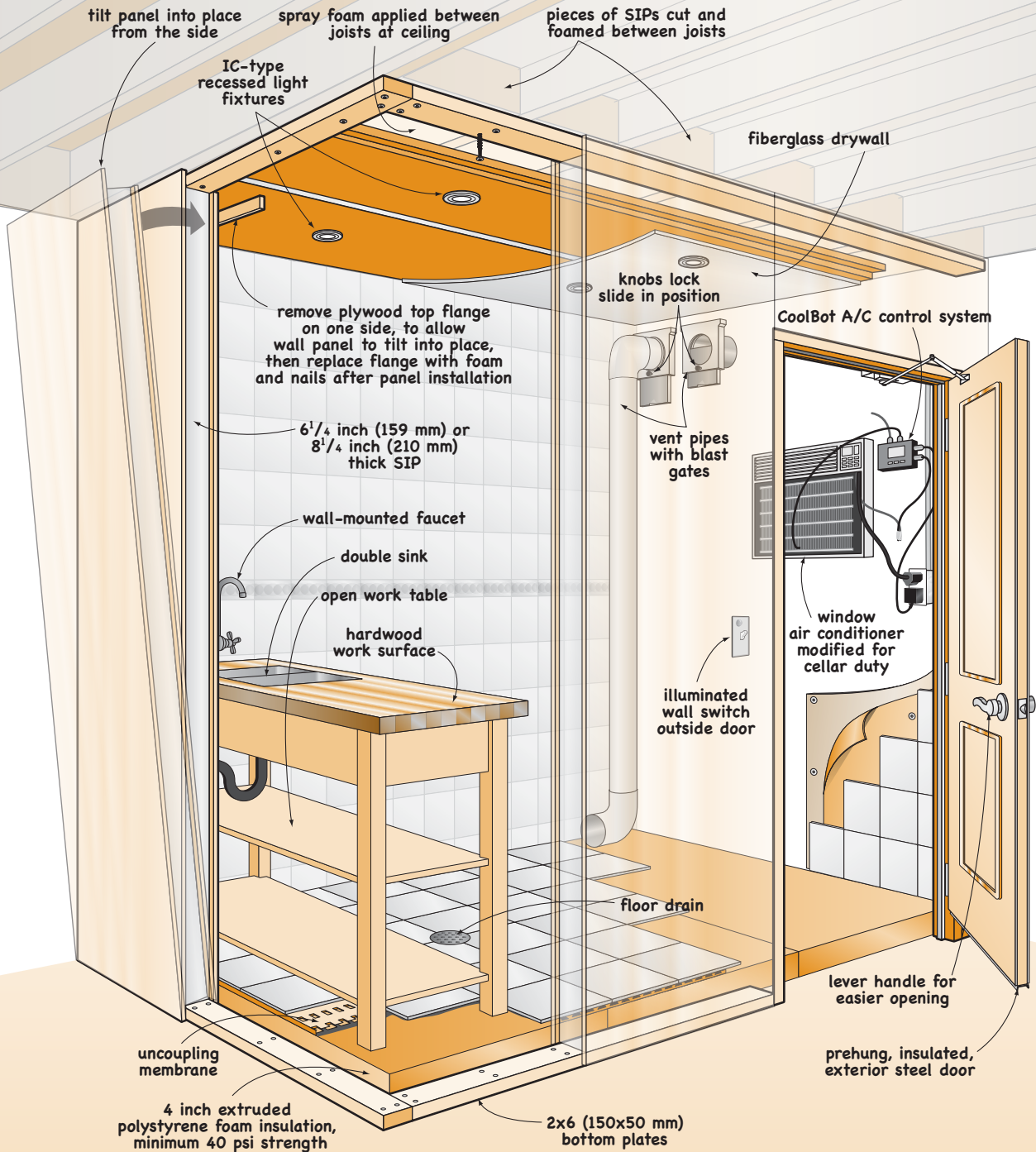
ELECTRIC ROOT CELLAR DETAILS
