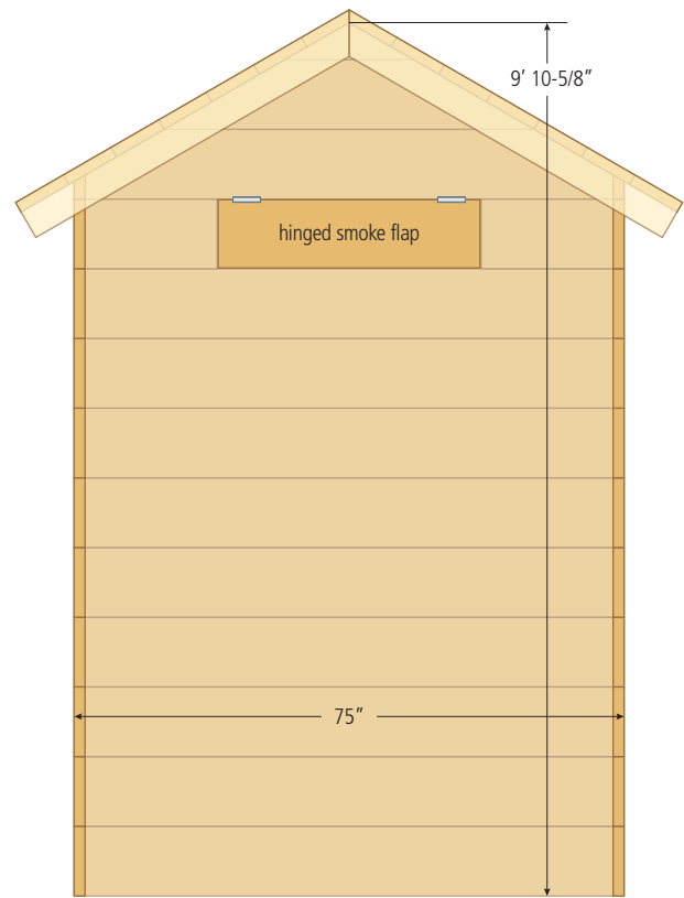
BACK VIEW
